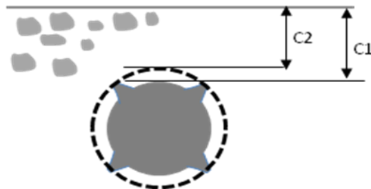
Gambar B.2 - Baja tulangan berusuk ( cm = C_2 )
