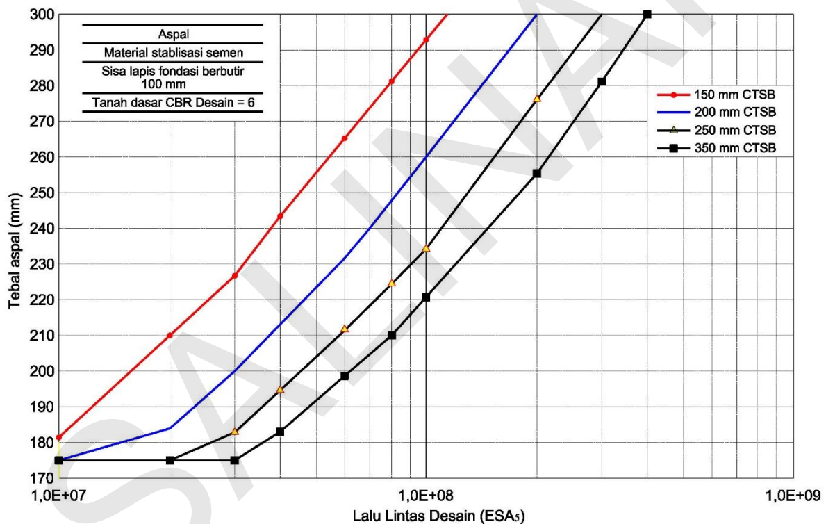
Gambar 8.4. Bagan Desain Ketebalan Cement Treated Recycled Base (CTR)
